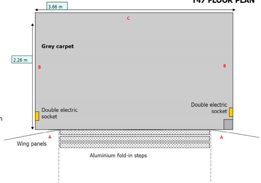
T47 FLOOR PLAN
